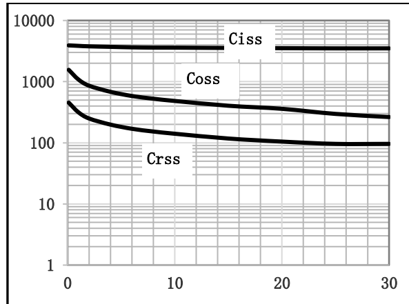
Fig.2 Capacitance Characteristics
